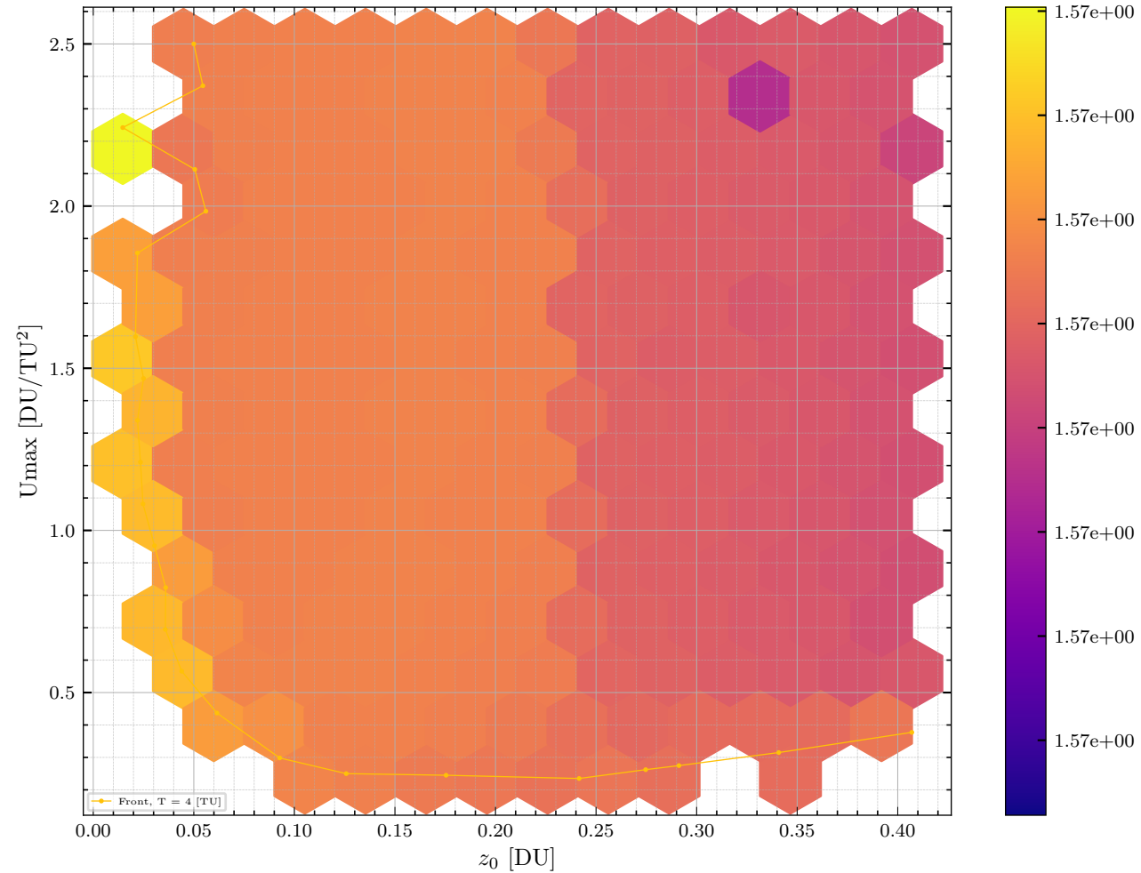
Cone angles [rad] over constant period, T = 4 [TU]
